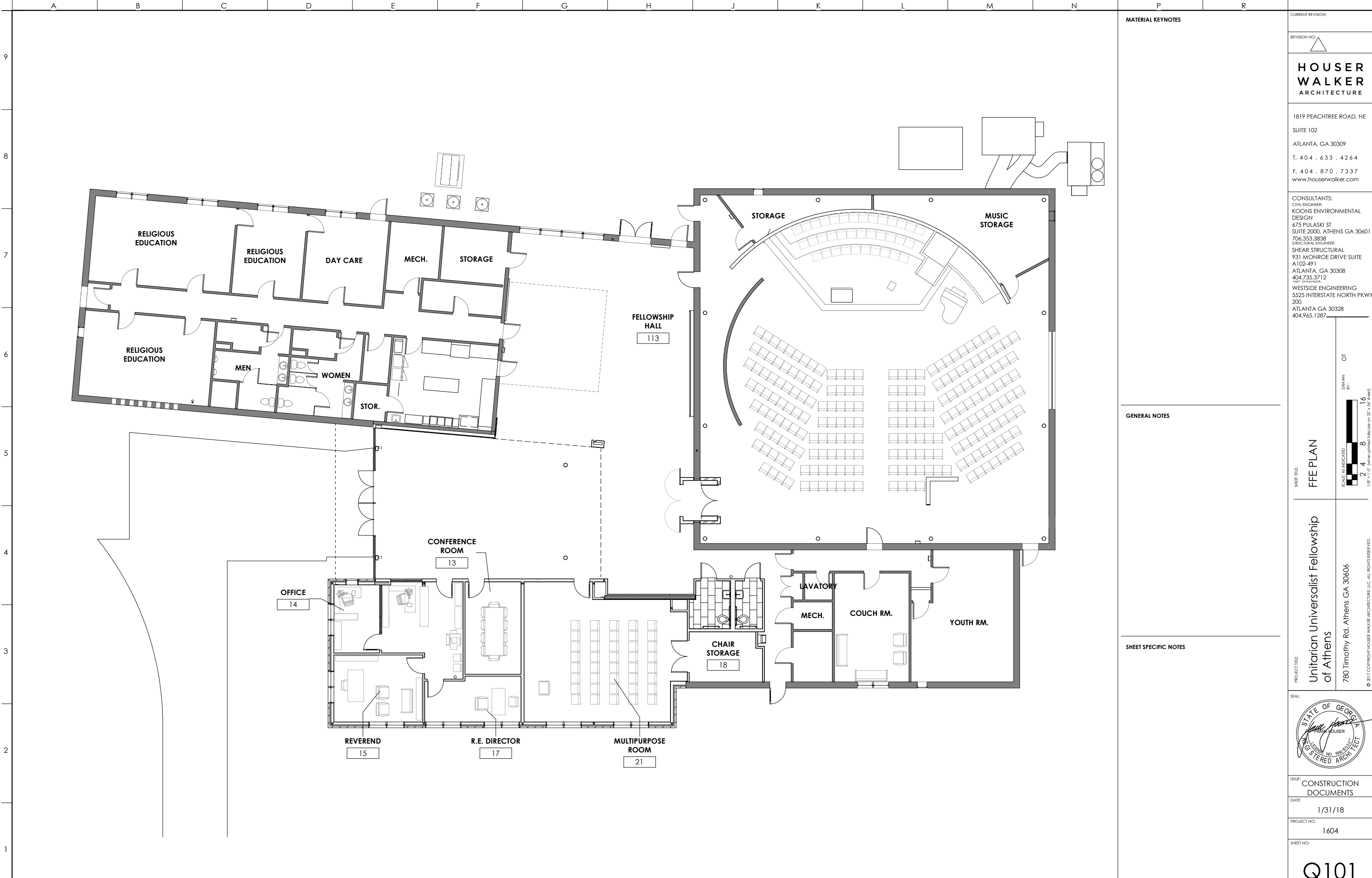
A1 FURNITURE PLAN
